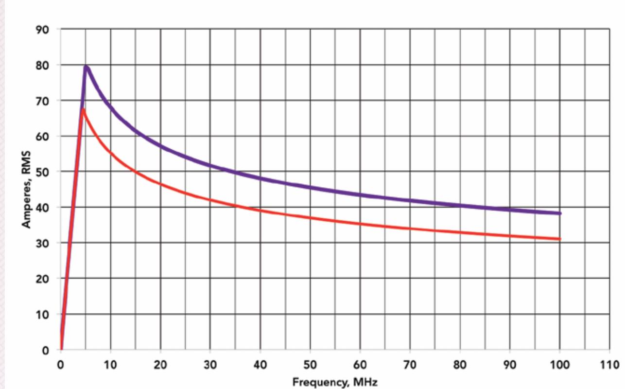
SIGIS RVVLA-1.8-1400-63 Maximum Working Current, Amperes Curves Derived from Voltage, ESR, and Cooling watts
