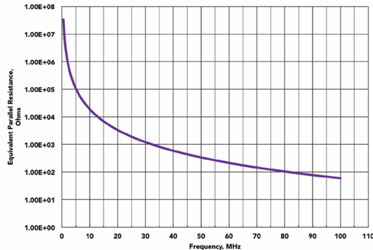
Equivalent Parallel Resistance vs. Frequency
