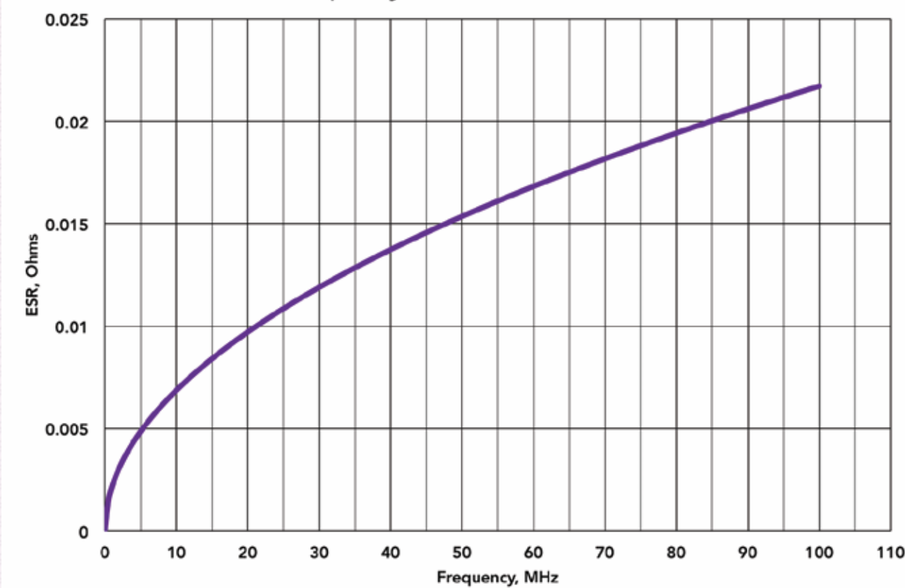
Frequency effective ESR, Ohms
